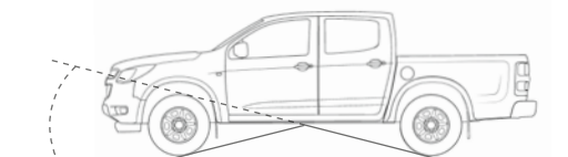
Ramp breakover angle
