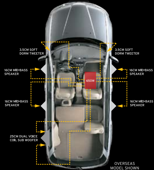
ROCKFORD FOSGATE® SPEAKER LOCATION
