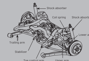
REAR SUSPENSION
