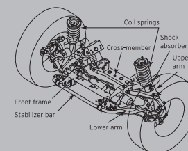
FRONT SUSPENSION
