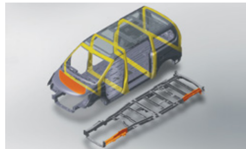
4 ring construction
