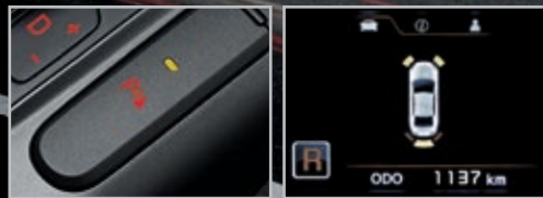
Front corner and rear parking assist system Activated by a switch on the floor console, (on A/T models, M/T models have a switch on the lower dash), the standard front corner and rear parking assist system shows the distance between the car and any obstruction by means of an in-cluster graphic display. (Some exterior colours come with black sensors).
