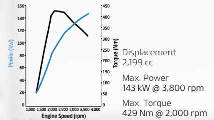
2.2L CRDi engine
