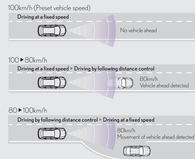
Radar Active Cruise Control
