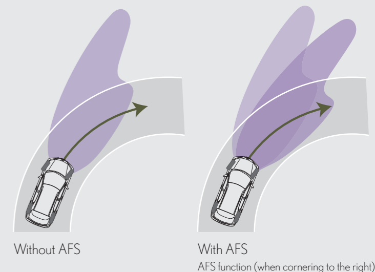
Active Front-lighting System (AFS)
