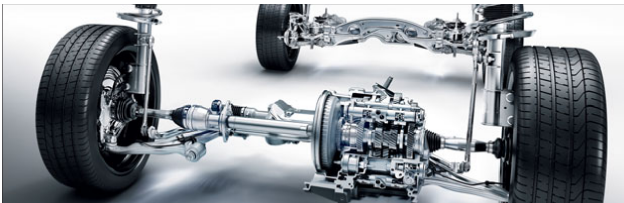
The new CLA is available with a suspension set up to provide a combination of sportiness and comfort or, optionally, for sporty driving
