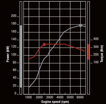
2.0L MIVEC DOHC Engine
