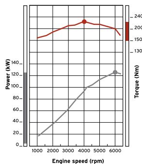
2.4L MIVEC Engine
