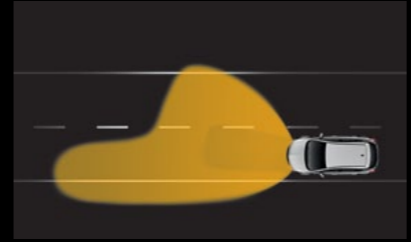
Adverse Weather Light (up to 70 km/h). Activated by wipers or a rain sensor, this setting improves vision in wet weather.
