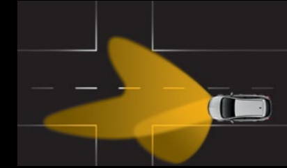
Static Cornering Light (up to 40 km/h, also works in reverse). Throws light 90° to the left or right, so you can better see what's around the corner.
