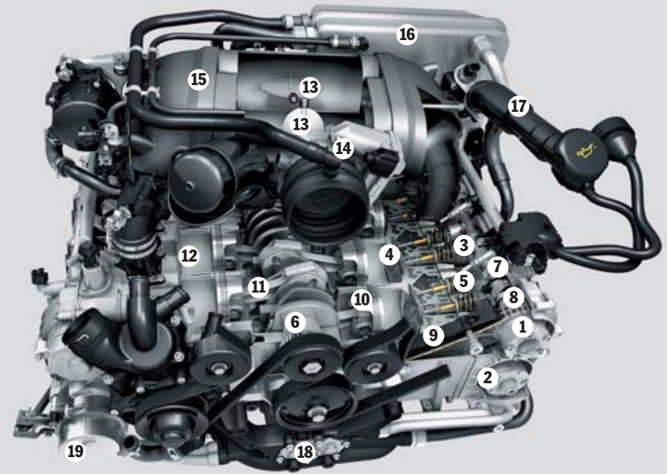
3.8-litre Boxer engine 911 GT3
