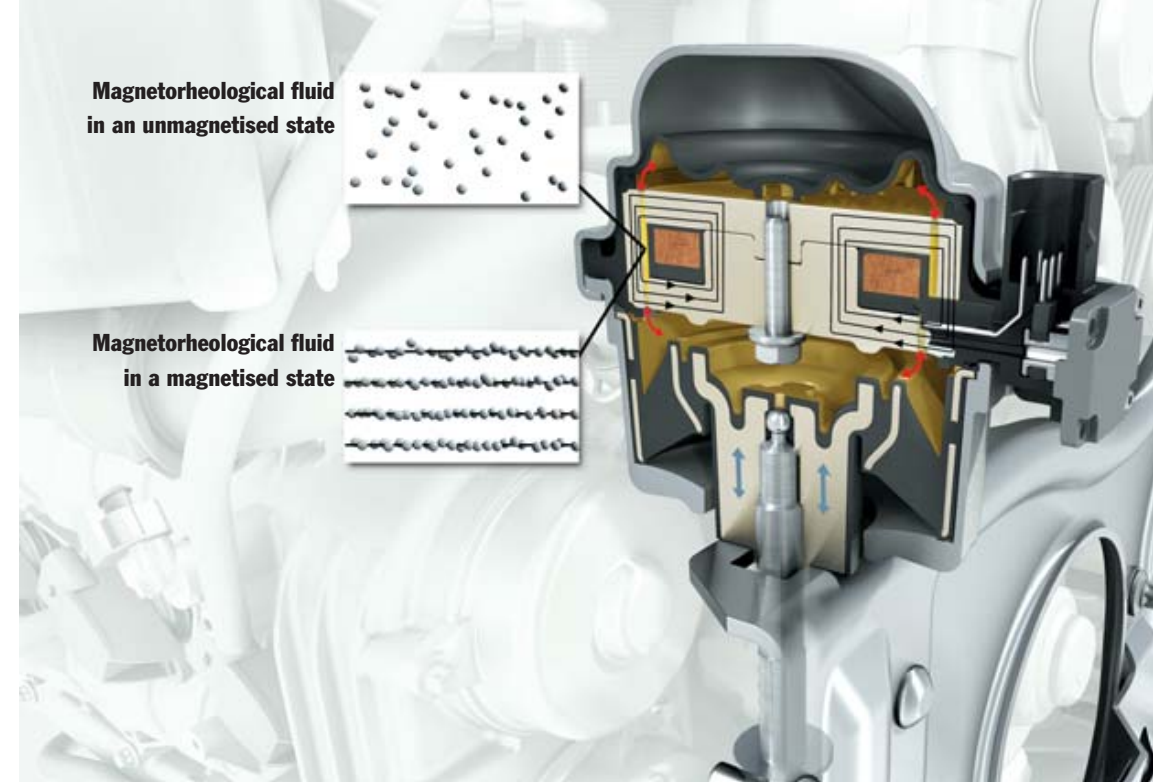
Dynamic engine mount system
