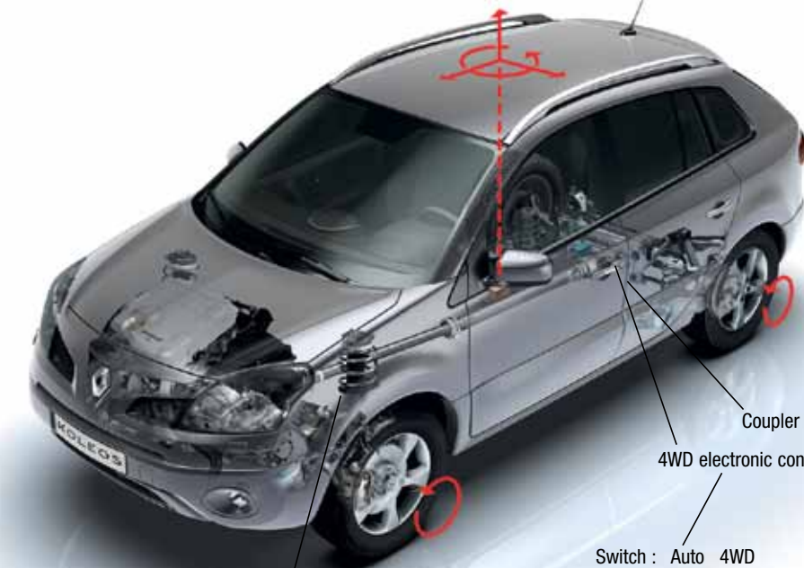
Wheel sensors (x4)
