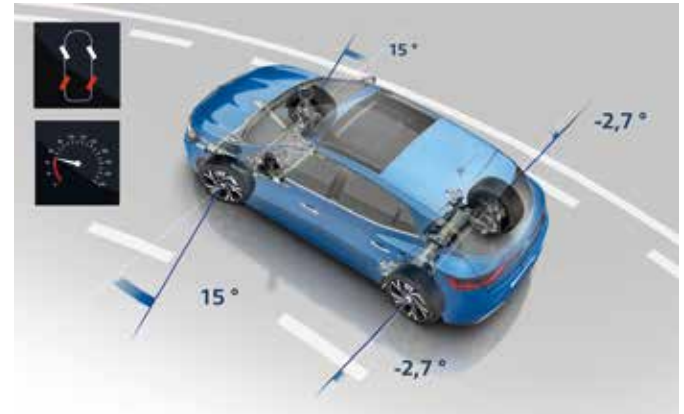
At low speeds of up to 60-80km/h, the rear wheels turn 2.7° in the opposite of the front wheels.
