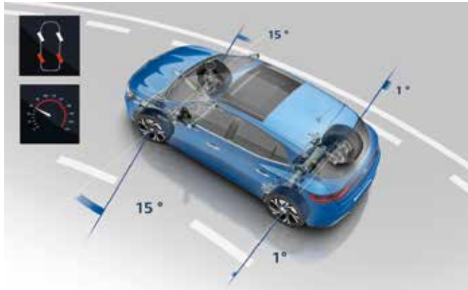
Above 80km/h, in Sport mode, the rear wheels turn in the same direction as the front wheel delivering unprecedented driver enjoyment and a driver experience that is both sporty and safe.
