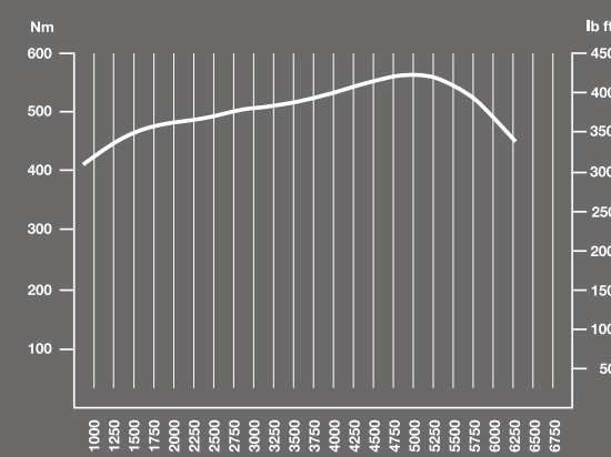
Torque
