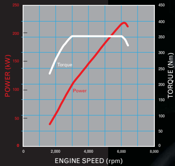
SUBARU WRX STI 2.5-LITRE FOUR-CYLINDER DOHC TURBOCHARGED BOXER PETROL ENGINE - AUTOMATIC TRANSMISSION 1
