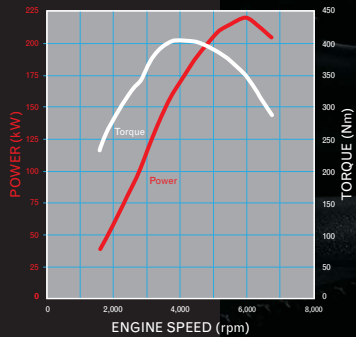
SUBARU WRX STI 2.5-LITRE, FOUR-CYLINDER DOHC TURBOCHARGED BOXER PETROL ENGINE - MANUAL TRANSMISSION 1
