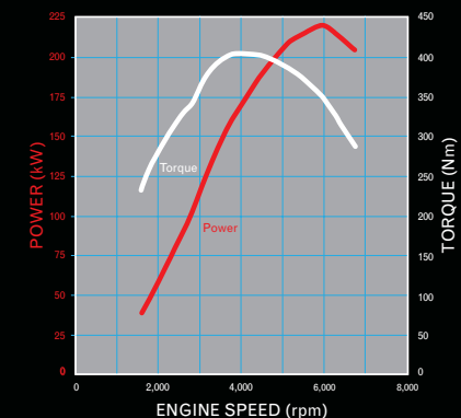
SUBARU WRX STI 2.5-LITRE, FOUR -CYLINDER DOHC TURBOCHARGED BOXER PETROL ENGINE - MANUAL TRANSMISSION 1
